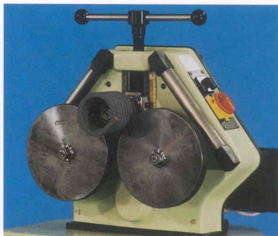
Oversized tooling can be used to roll very tight diameters, such as 1/2" square bar to a 3 inch I.D.
